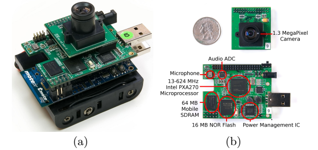
Figure 2: CITRIC camera mote. (a) An assembled camera daughter board with Tmote Sky board. (b) A camera daughter board with major functional units outlined.
