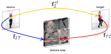
Figure 4: A path along the combined flows, \mathbf{f}_{IT} and \mathbf{f}_{TI} , should be consistent with a direct path along the \mathbf{f}_I^{st} .
