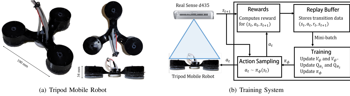
Fig. 1. (a) A soft mobile robot used in experiment. (b) A diagram for training system. The position of robot is measured by using blob detection from a RGB image of RealSense d435.
