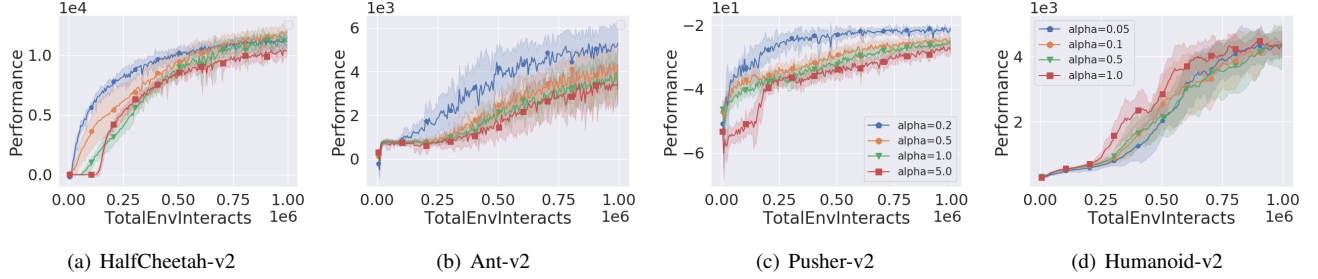
Fig. 3. ASAC with various initial entropy temperatures. (a), (b), and (c) share the legend.
