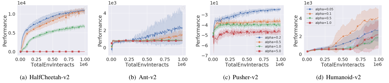
Fig. 2. SAC with various entropy temperatures. (a), (b), and (c) share the legend.
