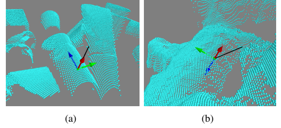
Fig. 3: Visualization of orthogonal bases at surface points sampled from the point clouds of cluttered objects. The red axes, blue axes, green axes indicate surface normal directions, major principal curvature directions, and minor principal curvature directions, respectively. Black lines indicate the surface normal directions computed by the standard principal component analysis. (a) A case of point cloud captured in the MuJoCo simulator [30]. (b) A case of point cloud captured by the RealSense depth sensor in the real world.
