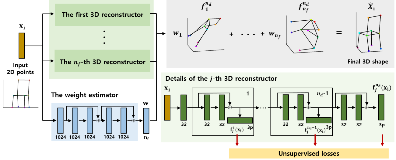
Figure 2. An overview of the proposed 3D shape reconstructor. It consists of n_f 3D reconstructors and a weight estimator. Here, each 3D reconstructor consists of n_d modules, and each module produces an intermediate reconstruction which is used in the intermediate losses to prevent the gradient vanishing problem. The reconstructions are weighted summed to estimate the final 3D shape. Here, the number written under each layer represents the channel size of the layer.
