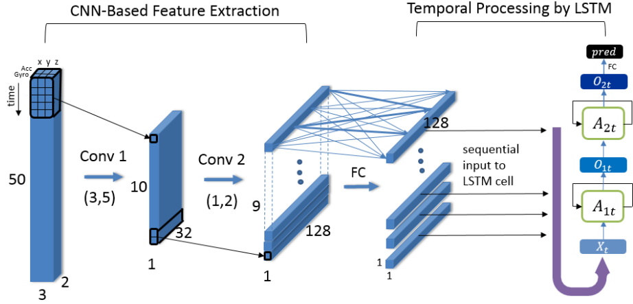
Fig. 4. The recurrent neural network structure used to recognize the gestures. Data dimensions and filter sizes are shown in the figure. Three-axes data of two sensors (accelerometer, gyroscope) are fed in the network. First, they pass through two convolutional layers and a fully connected layer. No padding for convolutional layers is used. Strides for two convolutional layer are five and one along time axis, respectively. A sequentially sliced vector is fed into two layers of stacked LSTM cells. The output of the last relevant cell according to the gesture sequence length is passed into a fully connected layer and results in a gesture prediction vector whose size is the number of gestures (nine in our case).
