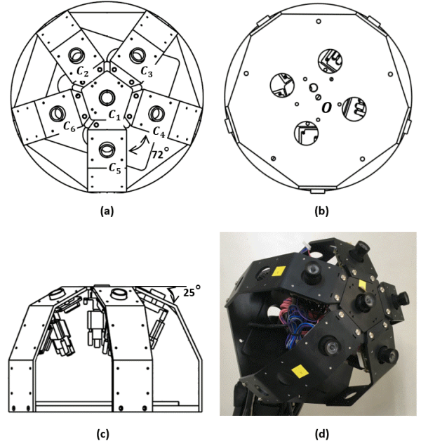
Fig. 1. The blueprints of the proposed device are visualized in (a) top view, (b) bottom view, and (c) side view. An image of the implemented hardware is shown in (d). It consists of six single-lens reflex camera modules, and they are synchronized.
