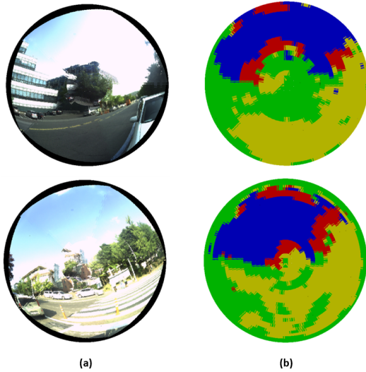
Fig. 7. Some examples of the semantic segmentation results on the real images. (a) compound mapped images, (b) inferred classes of each single image. Here, different colors mean different classes.
