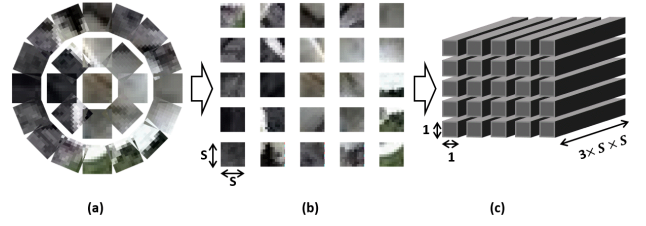
Fig. 4. (a) An example of the compound image configuration with the constraints. This example shows the case of n = 3 , (b) The single images on the hemisphere surface are considered to be on a flat square surface, (c) An illustration showing that each single image is vectorized to make it suitable for CNN.
