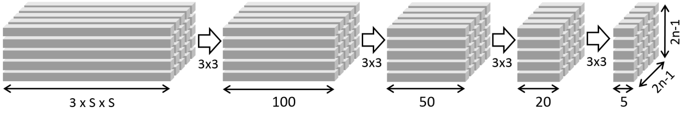
Fig. 3. A visualization of the proposed semantic segmentation network for compound images. It consists of four convolutional layers and a leaky ReLU activation layer is followed after each convolutional layer except the last layer. The output of the last layer is fed to the softmax layer to predict classes of each single image. In all convolutions, we use 3x3 size filters.
