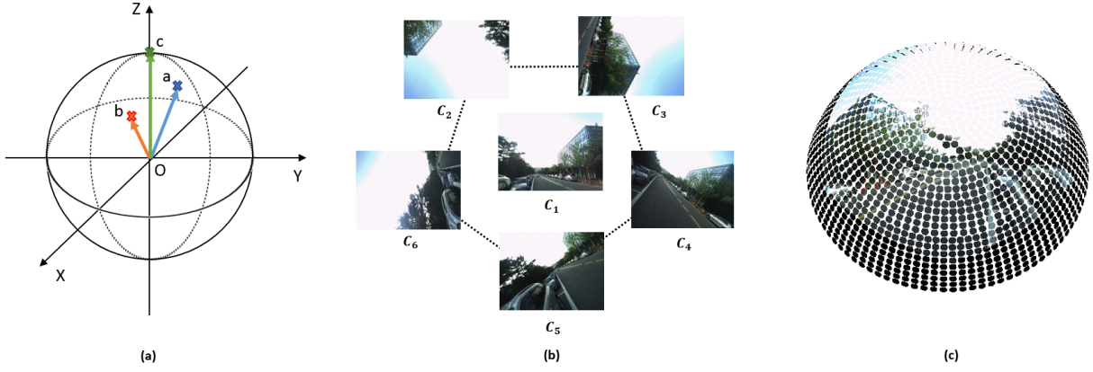
Fig. 2. A visualization of the compound eye's spherical coordinates, and an example of the proposed compound mapping scheme. (a) Three views of single eyes are visualized, (b) the images captured by the compound eye prototype, and (c) corresponding compound mapping results.
