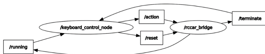
Figure 1. Nodes and topics illustrated by ' rqt_graph '.
