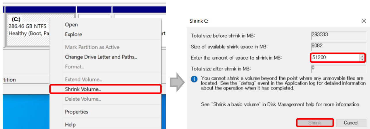
Figure3. Disk Partition
