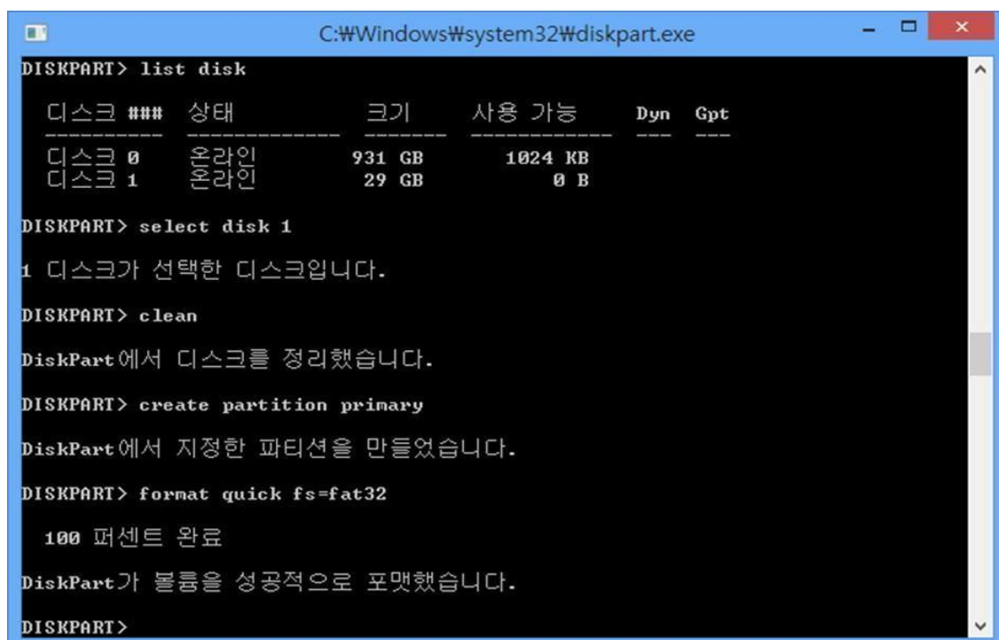
Figure 1. Prior setting for making booting USB
