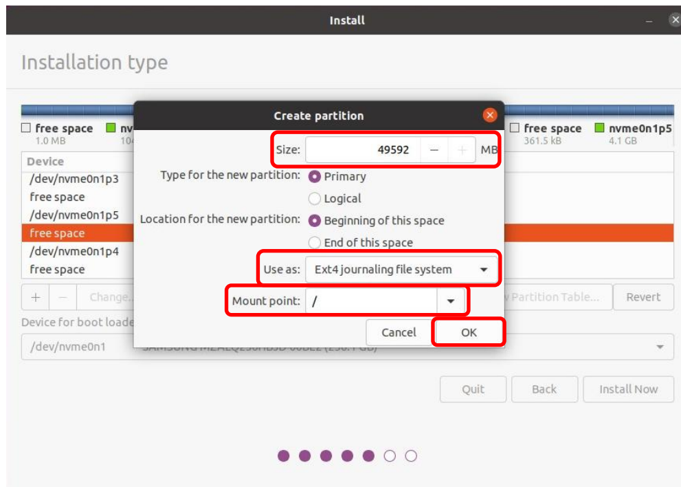
Figure 5. Root partition allocation for Installation of Ubuntu 20.04 LTS
