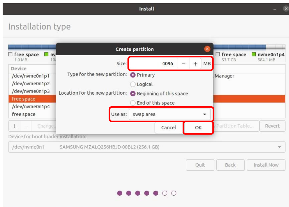
Figure 6. Swap partition allocation for Installation of Ubuntu 20.04 LTS
